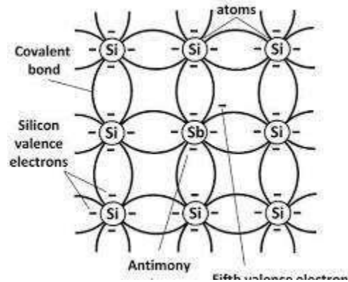
N-type semiconductor doping diagram
