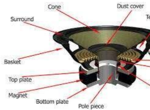
Speaker showing a magnet
