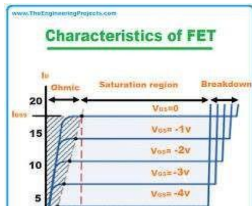
FET output characteristics graph
