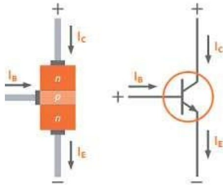
BJT structure diagram
