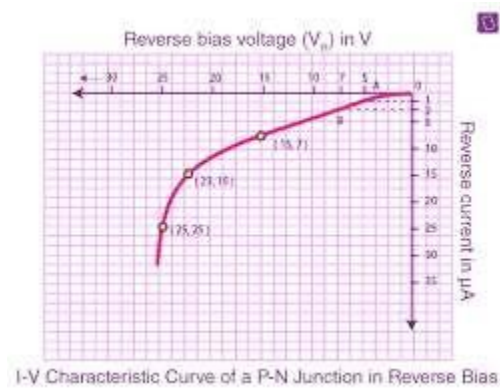
Diode's reverse bias IV curve
