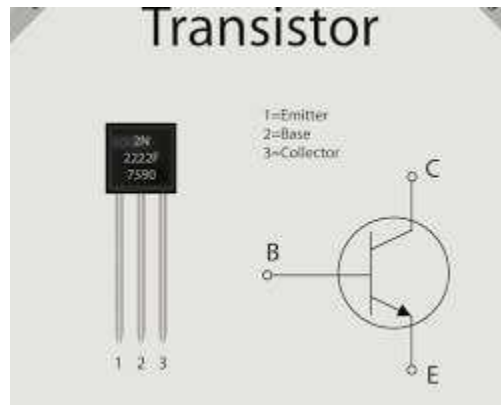
Transistor
