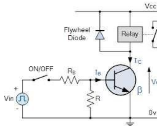
Assembled transistor switching circuit
